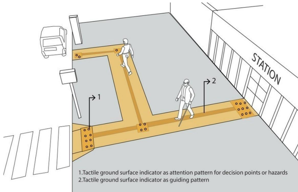
Figure 15 Typical Representation of TGSi in Transit Areas
